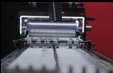
Shingle stream delivery table for sheeted labels
