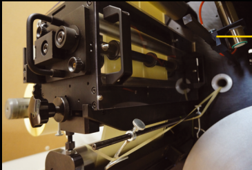
Cassette type slitting system: shear cutting, razor cutting and crush cutting
