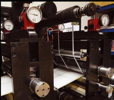
Servo controlled die cutting station with pressure gauges
